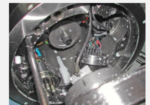
Fault rotary union and consequential damages
